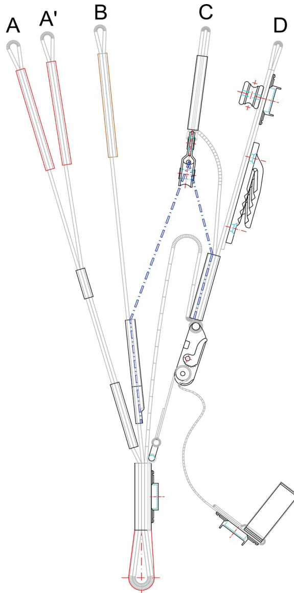
Figure: 20 mm webbing risers (standard)
