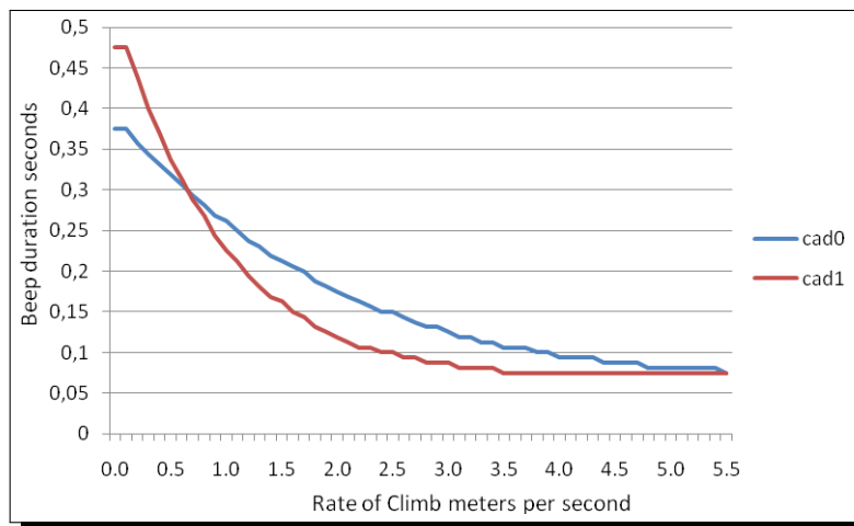
Figure 4.23: Cadence timing
